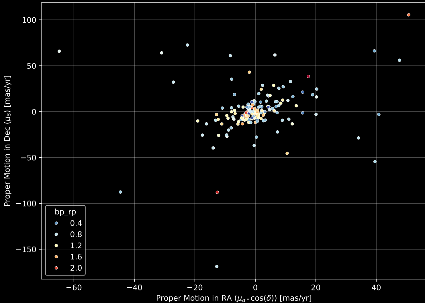
APOGEE DR17 Field: [CVZ_OB03_btx] Proper Motion Diagram (n= 179)
