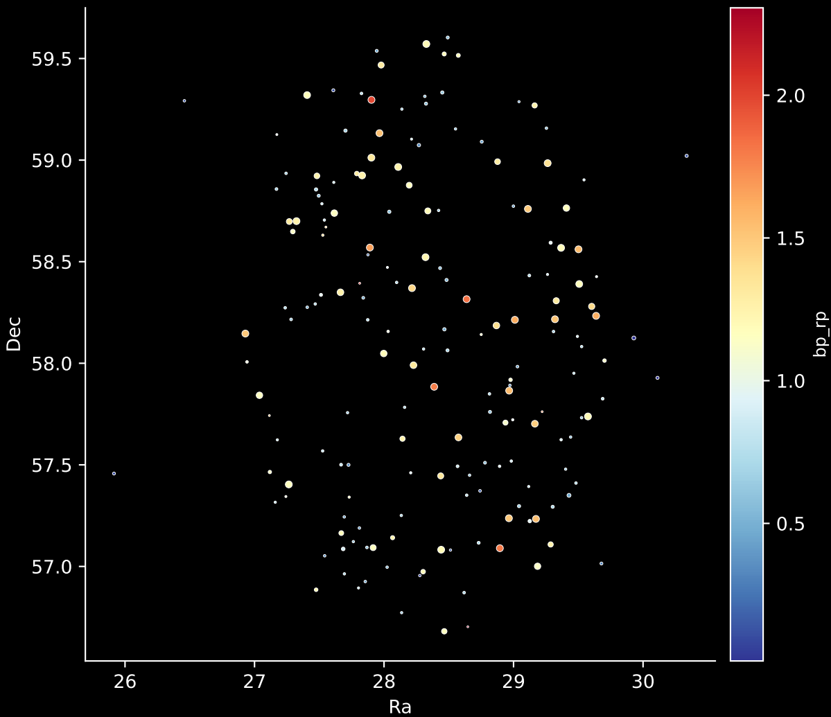
APOGEE DR17 Field: [CVZ_OB03_btx] Stars: 179
