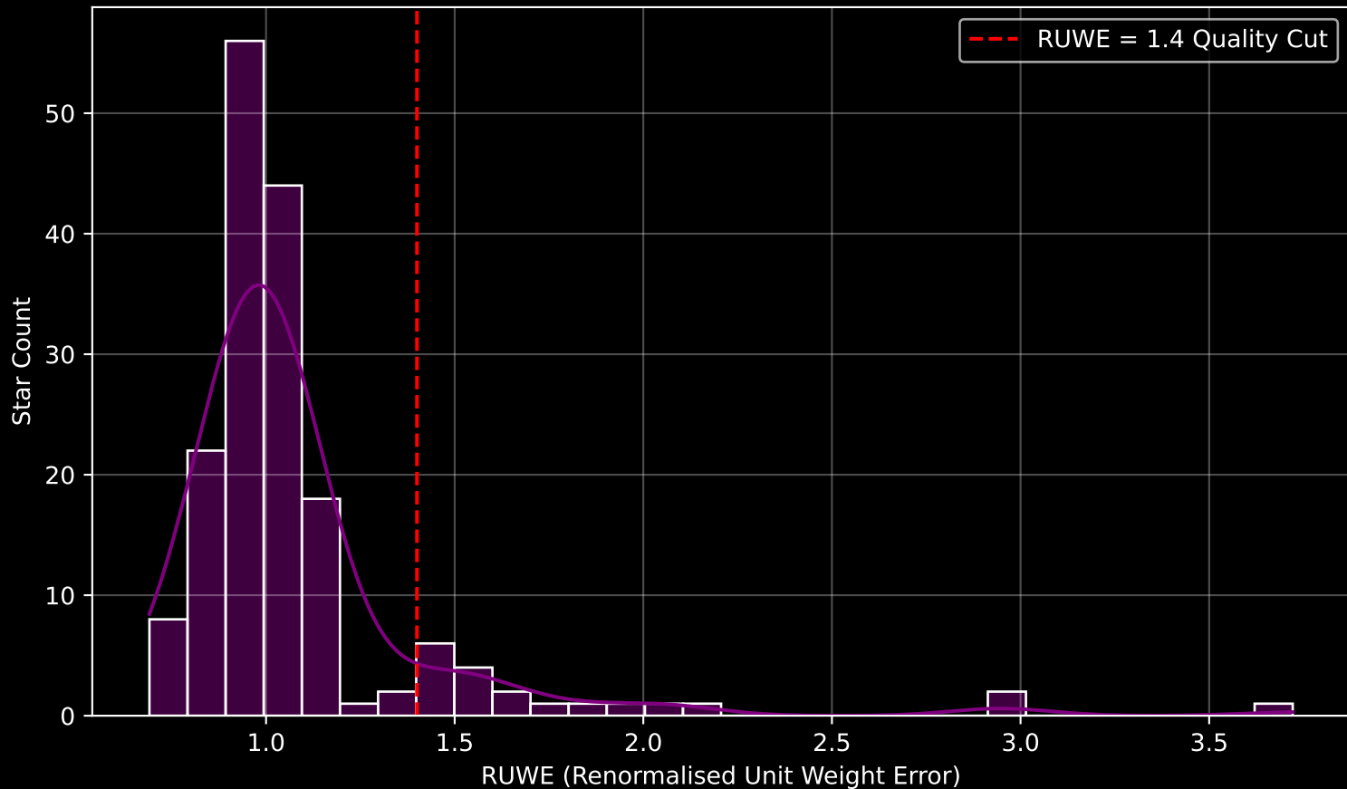
GAPOGEE DR17 Field [CVZ_OB03_btx] RUWE Distribution (n= 171)
