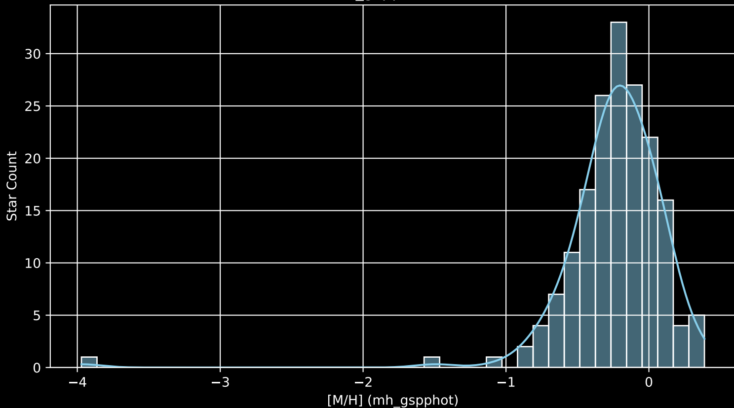
APOGEE DR17 Field: [CVZ_OB03_btx [M/H] (mh_gspphot) (n= 177)
