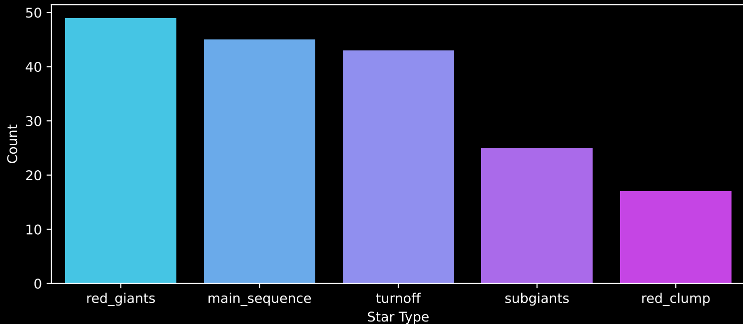
APOGEE DR17 Field: [CVZ_OB03_btx] Count plot of Star Type
