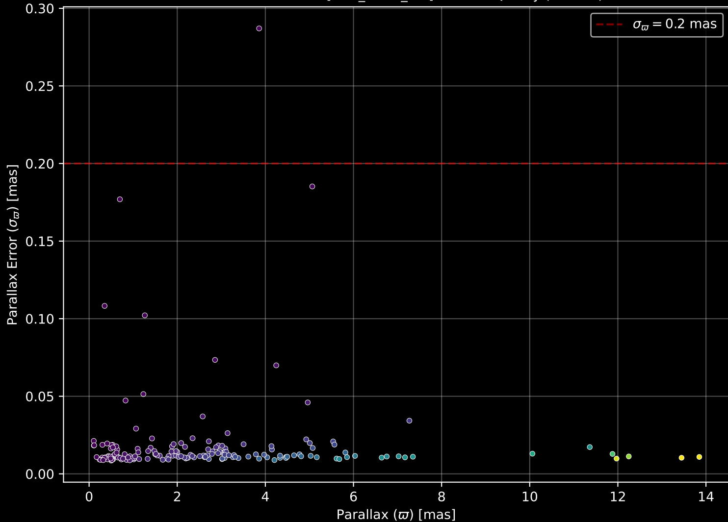
APOGEE DR17 Field: [CVZ_OB03_btx] Parallax Quality (n= 179)
